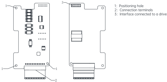
Fig. 1 PG*1S appearance (for models of 3.7 kW and below)
