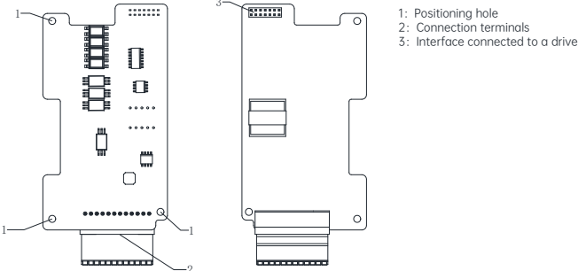
Fig. 2 PG*1S appearance (for models of 5.5 kW and above)
