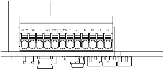
Fig. 3 Terminal mark
