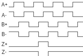
Fig. 4 ABZ signal
